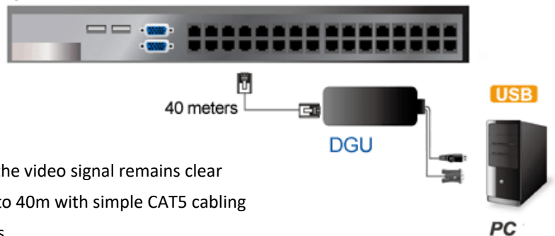
CAT5 KVM 8/16/32 Port
