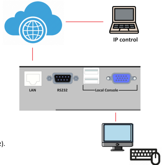
Rear of KVM-1708/1908AST-M2-BIP
