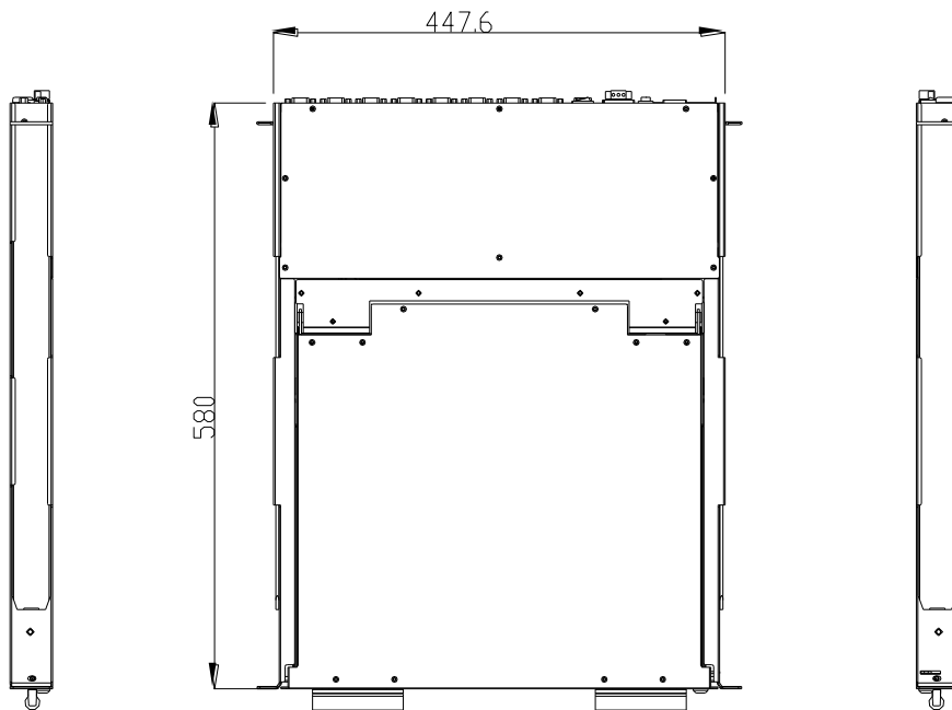
Rear of KVM-1732W-ASL-M2/ULC
