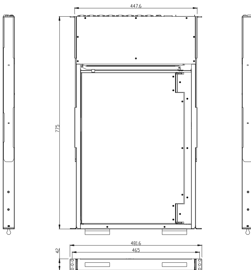
Rear of KVM-2132/2432ASL-M2/ULC
