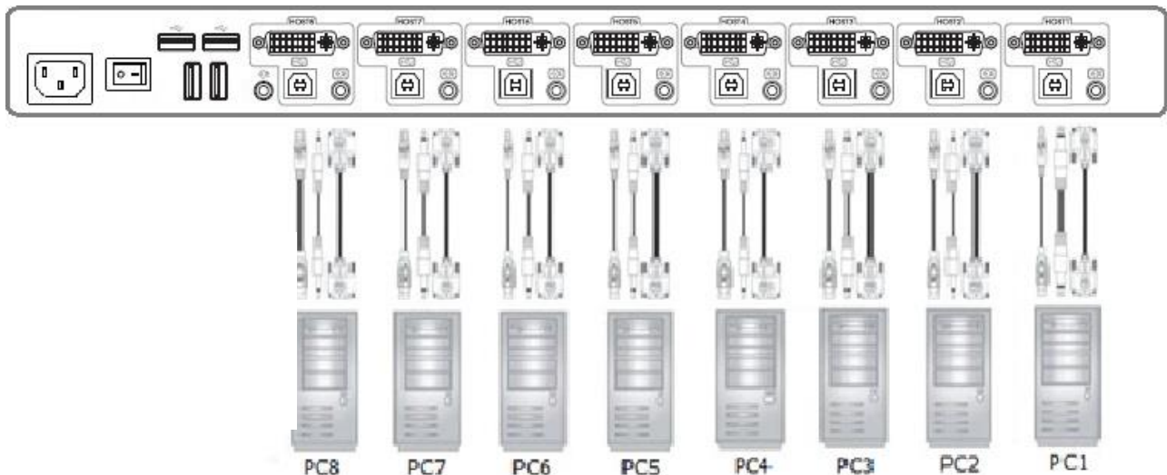
Figure 3. Computer/Server Installation
