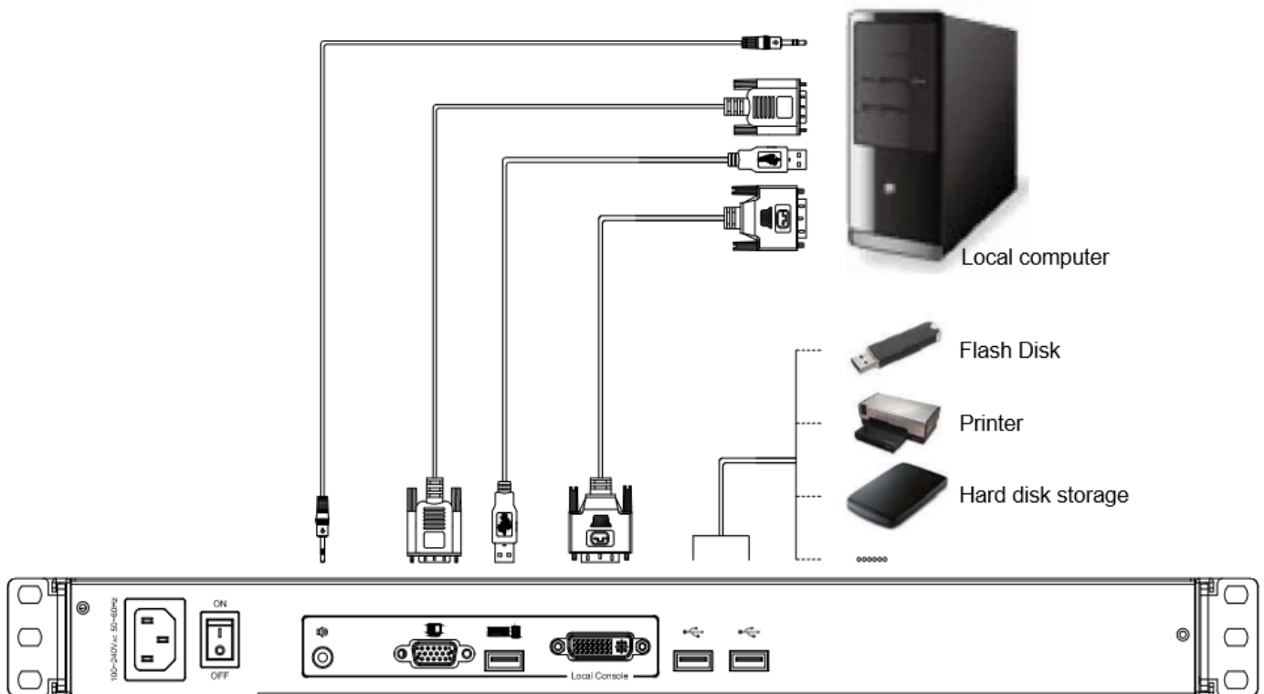
KVM-1701SWPD-REAR-COVER
