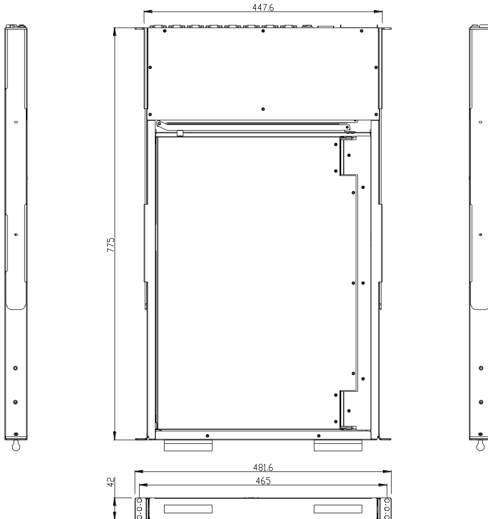
Rear of KVM-2101WPD-M2
