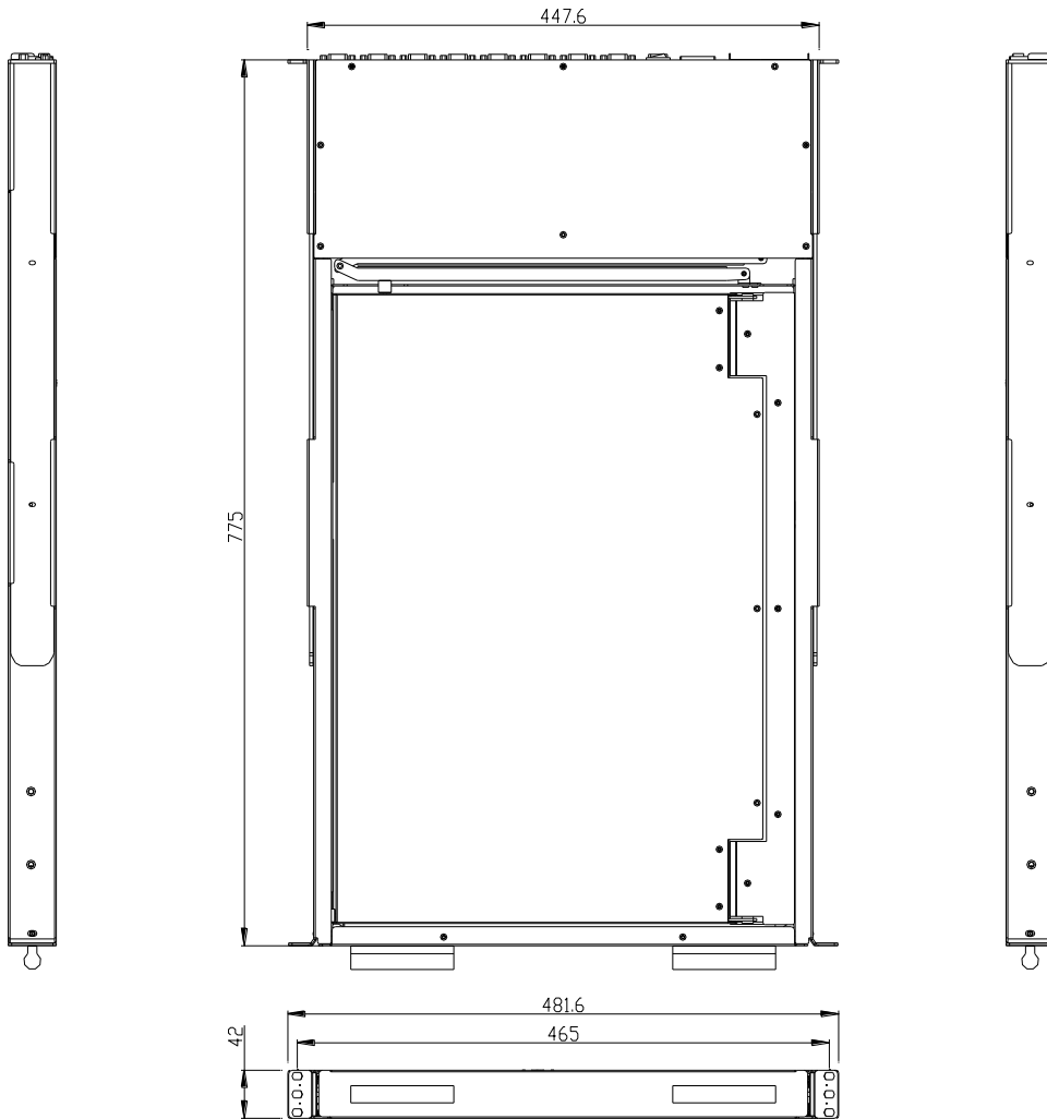
Rear of KVM-2401WPD-M2
