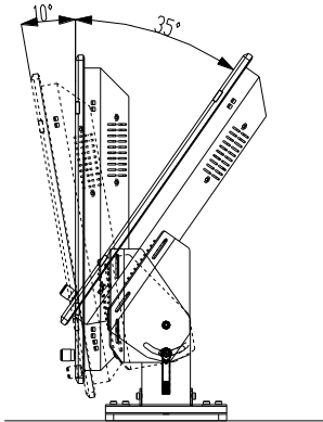
Stand mount
