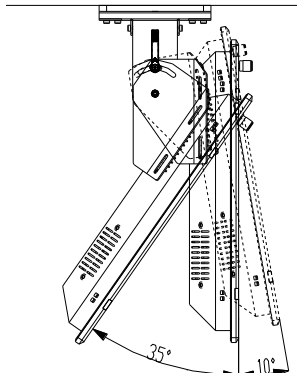
ROOF mount
